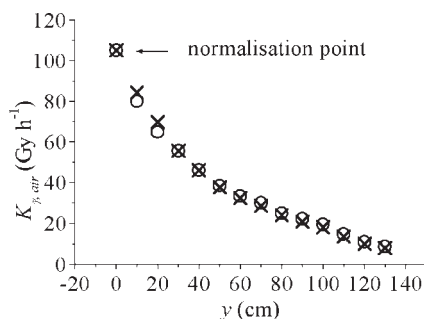
Figure 4. Axial photon dose profile in the fast neutron beam (open circle, calculated values; cross, measured values). The measurements were performed using D-3 TLDs and the calculated values were normalised to a measurement point.
