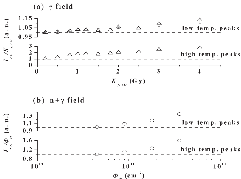
Figure 5. Sensitivity of TLD-100 as a function of photon kerma in air and thermal neutron fluence. Except for the low temperature peaks in the pure photon field, the uncertainties were omitted since they are smaller than the symbol size.
