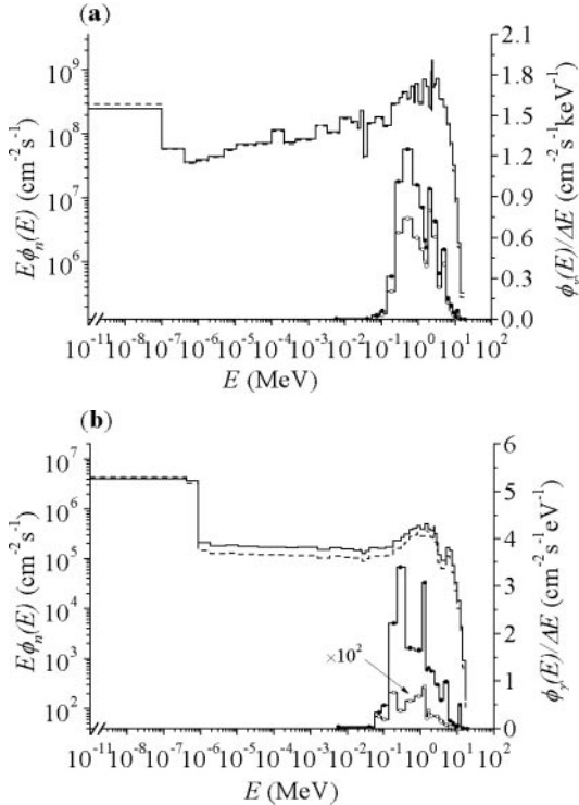
Figure 1. Spectra of neutron fluence rate per unit lethargy and calculated spectra of photon fluence rate per unit energy in the (a) fast and (b) thermal neutron beams (dashed line (---) calculated neutron spectra; straight line (—) adjusted neutron spectra; lines joining open circles: photon reactor background; lines joining closed circles: total photon) in the irradiation facilities.
