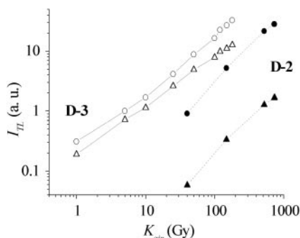
Figure 3. Relative TL intensity of \text{Al}_2\text{O}_3\text{:Mg,Y} detectors D-2 and D-3 as a function of photon kerma in air (circles, low temperature peak; triangles, high temperature peak).
