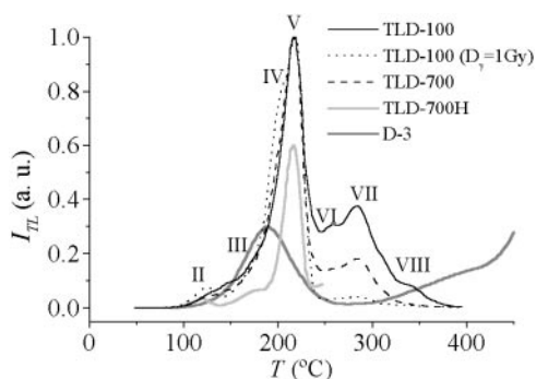
Figure 2. Glow curves (not to scale) of TL materials irradiated in a mixed radiation field of thermal neutrons (thermal neutron fluence: 3 \times 10^{11} \text{ cm}^{-2} ) and photons (air kerma: 200 mGy). The glow curve peaks of LiF:Mg,Ti are identified by roman numerals.
