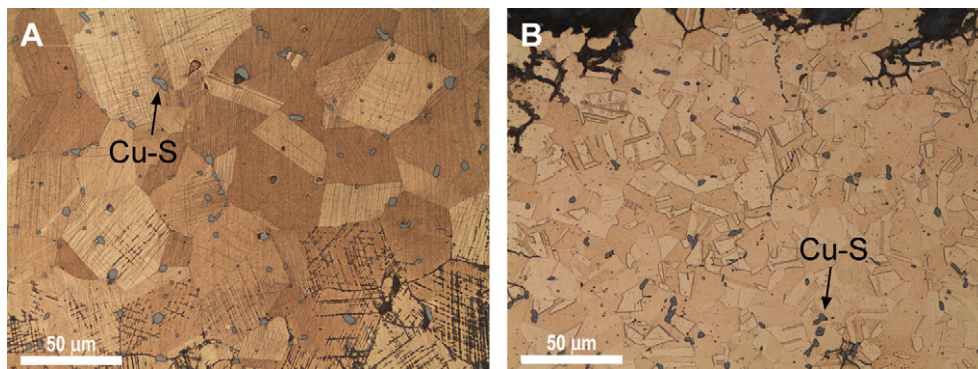
Fig. 5. Microstructures of (A) needle CRAT05/C1/Ib/M2 and (B) needle CRAT07/R1/IIc/M1 (BF-cross-section, etched).
