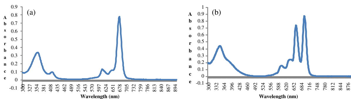
Figure 1. UV-vis spectra of phthalocyanines 7 (a) and 8 (b) recorded in \text{CH}_2\text{Cl}_2 .
