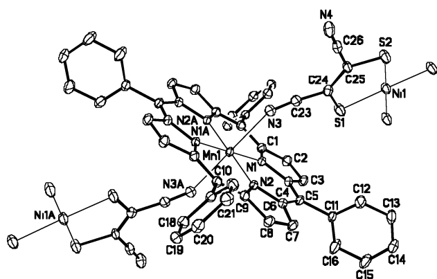
Figure 2. ORTEP atom-labeling diagram of [\text{MnTPP}]\{\text{Ni}[\text{S}_2\text{C}_2(\text{CN})_2]\}_2 , 4 , complexes using 30% thermal ellipsoids.
