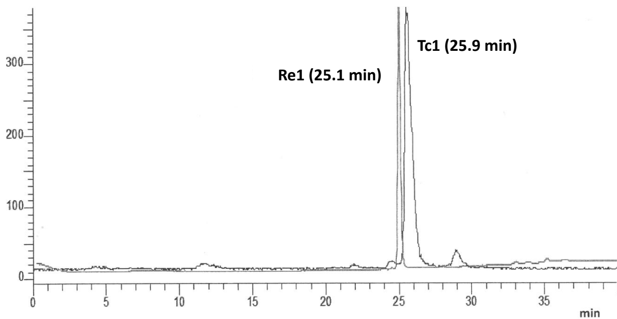
Figure S6. RP-HPLC analytical chromatograms of Re1 (UV detection, 220 nm) and Tc1 ( \gamma -detection).
