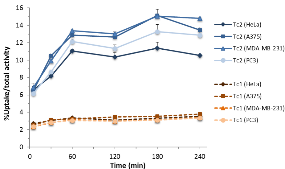
Figure 1. Cellular uptake of Tc1 and Tc2 in human cancer cell lines at 37°C.
