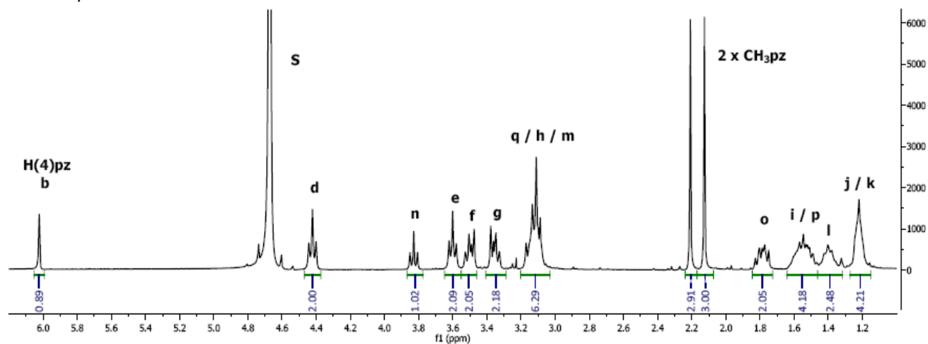
1 H-NMR spectrum
