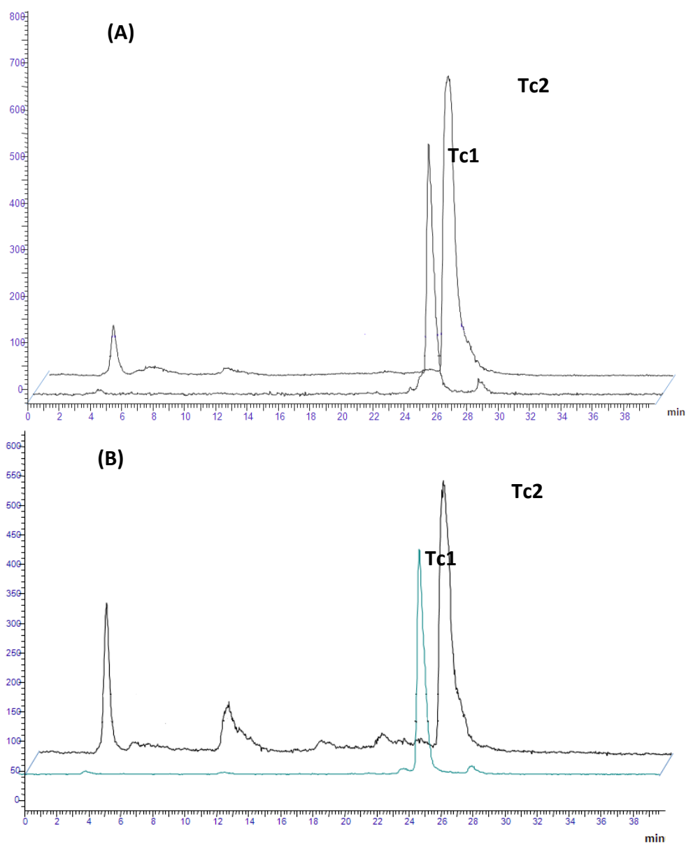
Figure S5. Stability of Tc1 and Tc2 . RP-HPLC chromatograms of Tc1 and Tc2 in phosphate buffered saline (PBS) pH 7.4 (A) and in PBS pH 7.4 with a 100 fold excess histidine (B) after 24 h at 37°C. Macherey-Nagel C18 reversed-phase column (Nucleosil 100-5, 250 x 3 mm) with a flow rate of 0.5 mL/min. Eluents: aqueous 0.1 % CF 3 CO 2 H/MeOH. Gradient: t = 0-5 min: 10 % MeOH; 5-30 min: 10→100 % MeOH; 30-34 min: 100 % MeOH; 34-35 min: 100→10 % MeOH; 35-40 min: 10 % MeOH. \gamma detection.
