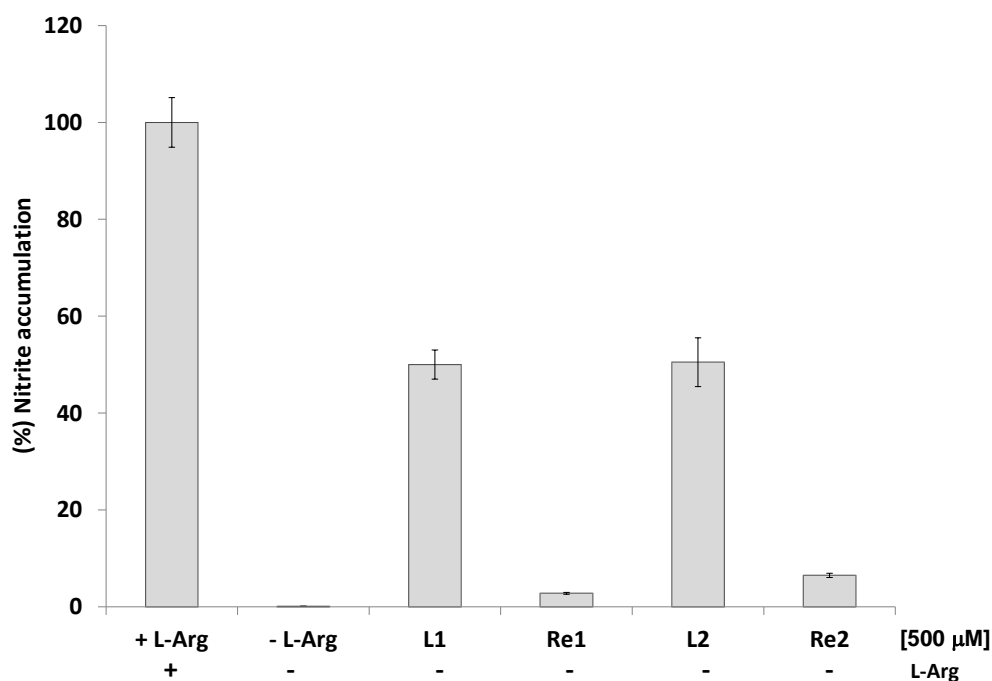
Figure 6: Effect of L1 , L2 , Re1 and Re2 on NO biosynthesis by LPS-induced RAW 264.7 macrophages. Data are expressed as % of nitrite accumulation of the L-Arg control (mean \pm S.D. -standard deviation, n = 8). The experiment was repeated three times with comparable results
