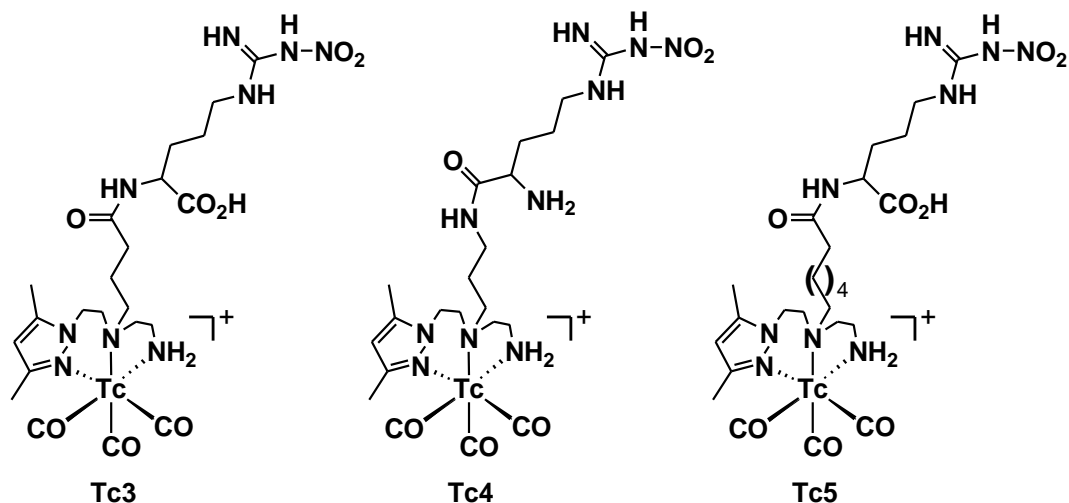
Scheme 2. Molecular structures of Tc3 - Tc5 .
