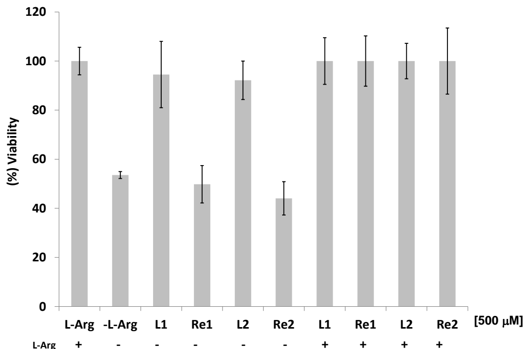
Figure 7- Viability in macrophages RAW 264.7 incubated with the compounds, in the absence or presence of L-arginine in the culture medium. Viability of cells incubated with LPS and L-arginine was considered as 100 % (mean \pm S.D., n = 8). This experiment was repeated two/three times with comparable results.
