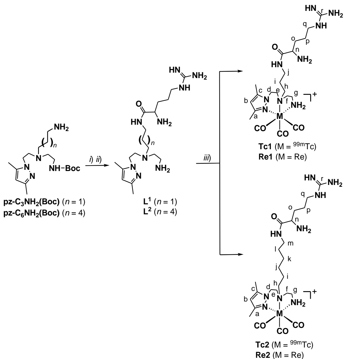
Scheme 1. Synthesis of \text{L}^1 , \text{L}^2 , \text{Tc1/Re1} and \text{Tc2/Re2} (Identification system for NMR assignments is displayed for the rhenium complexes). i) \text{Et}_3\text{N} , N - \alpha -Boc-L-Arg, HBTU, 2 h, r.t.; ii) \text{CH}_2\text{Cl}_2 -TFA, 3 h, r.t.; iii) [\text{M}(\text{CO})_3(\text{H}_2\text{O})_3]^+ ( M = \text{Re} , {}^{99\text{m}}\text{Tc} ), \text{H}_2\text{O} , 100^\circ\text{C} .
