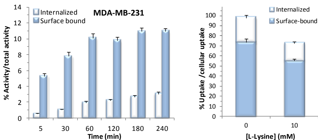
Figure 3. A) Internalized and surface-bound Tc2 in HeLa, A375 and MDA-MB-231 cancer cell lines at 37°C, expressed as a percentage of total applied activity. B) Internalized and surface-bound Tc2 after 2 h in the presence of lysine at 37°C, expressed as a percentage of cellular uptake in the absence of L-Lys.
