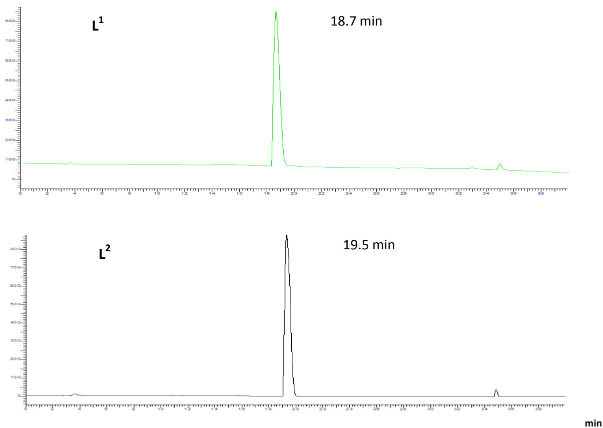
Figure S1. RP-HPLC chromatograms of L 1 and L 2 . Macherey-Nagel C18 reversed-phase column (Nucleosil 100-5, 250 x 3 mm) with a flow rate of 0.5 mL/min. Eluents: aqueous 0.1 % CF 3 CO 2 H/MeOH. Gradient: t = 0-5 min: 10 % MeOH; 5-30 min: 10→100 % MeOH; 30-34 min: 100 % MeOH; 34-35 min: 100→10 % MeOH; 35-40 min: 10 % MeOH. Detection: \lambda = 220 nm.
