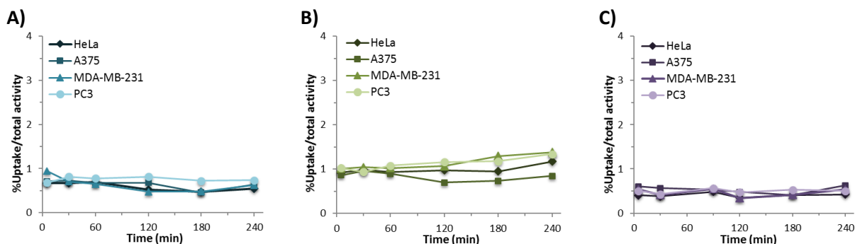
Figure 2. Cellular uptake of the radioconjugates Tc3 (A), Tc4 (B) and Tc5 (C) in various human cancer cell lines at 37°C.
