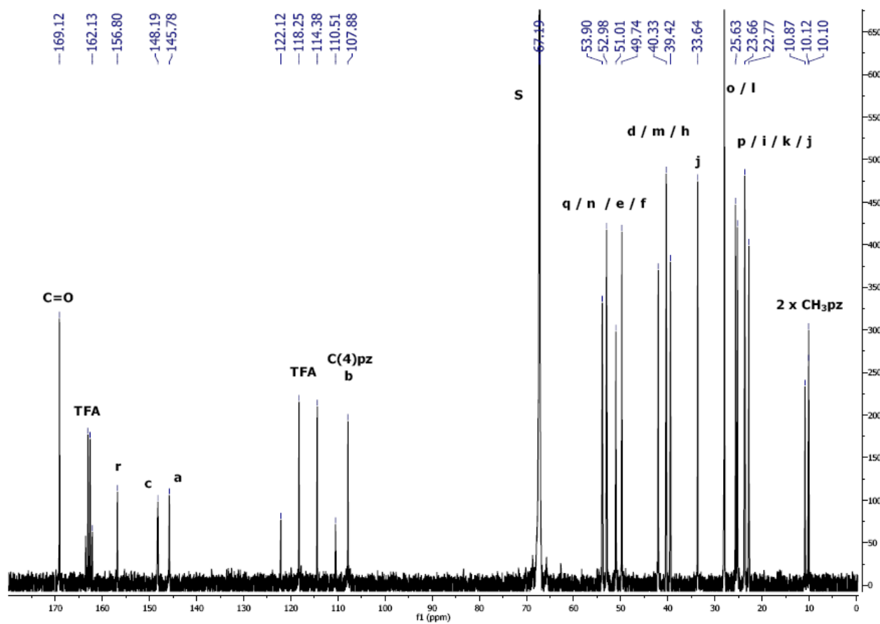
Figure S3. Assigned 1 H and 13 C-NMR spectra of L 2 .
