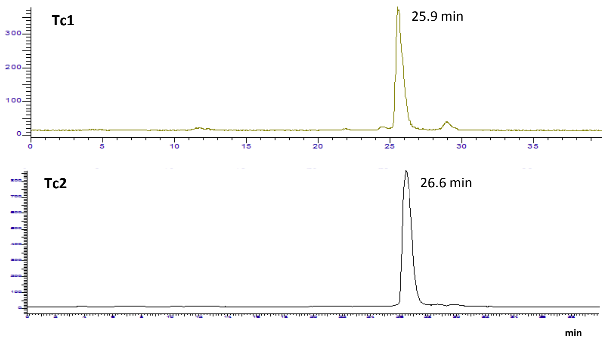
Figure S4. RP-HPLC chromatograms of Tc1 and Tc2 . Macherey-Nagel C18 reversed-phase column (Nucleosil 100-5, 250 x 3 mm) with a flow rate of 0.5 mL/min. Eluents: aqueous 0.1 % \text{CF}_3\text{CO}_2\text{H} /MeOH. Gradient: t = 0-5 min: 10 % MeOH; 5-30 min: 10 \rightarrow 100 % MeOH; 30-34 min: 100 % MeOH; 34-35 min: 100 \rightarrow 10 % MeOH; 35-40 min: 10 % MeOH. \gamma detection.
