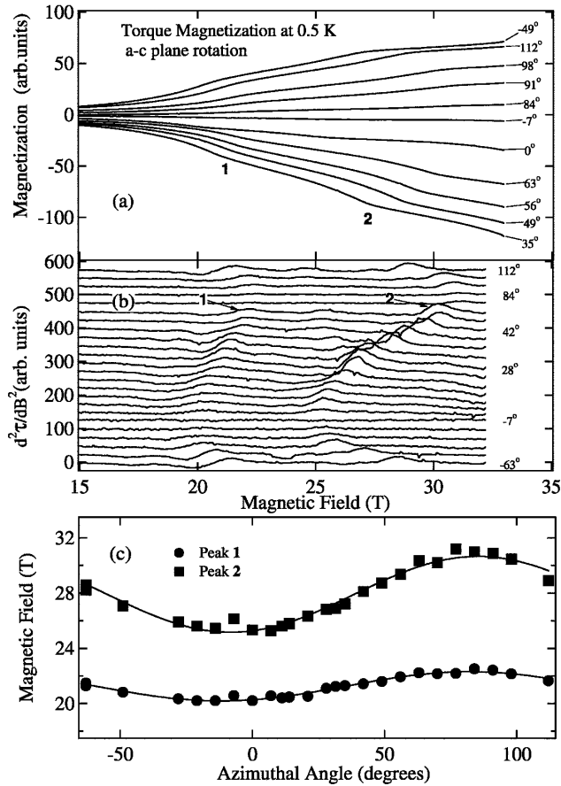
FIG. 3. Magnetization of (\text{Per})_2\text{Pt}(\text{mnt})_2 at 0.5 K up to 33 T. (a) Torque magnetization signal \tau/B for a sample rotated in the a-c plane with respect the magnetic field. Transitions 1 and 2 in the field range 20 to 30 T are indicated. (b) The second derivative of the torque signal |d^2\tau/dB^2| vs field and angle. (c) a-c plane angular dependence of the main magnetization signals 1 and 2 . Lines are sinusoidal fits to the data.
