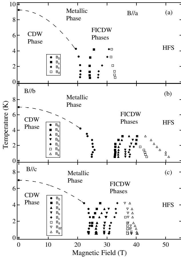
FIG. 2. Proposed T-B phase diagram of (\text{Per})_2\text{Pt}(\text{mnt})_2 based on the magnetoresistance studies in Fig. 1. Features of the magnetoresistance noted as B_o , B_x , and B_e indicate the suppression of the low field CDW state, the onset and termination of the FICDW state, respectively. Cascadelike properties of the magnetoresistance are identified as B_a , B_b , B_c , and B_d where closed symbols are below and open symbols are above the center of the FICDW. Dashed lines: quadratic extrapolation between T_c(0) and T_c(B_0) . (a) B//a phase diagram based on Fig. 1(a). (b) B//b phase diagram based on Fig. 1(b). Note that the upper phase boundary B_e is an estimate based on a linear extrapolation of the data to fields above 45 T. (c) B//c phase diagram based on Fig. 1(c).
