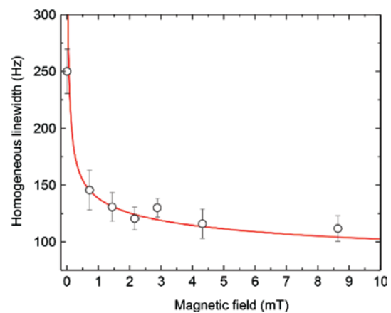
Figure 3: Nuclear spin homogeneous linewidth of ^{151}Eu^{3+}:Y_2O_3 ( \pm 1/2 \rightarrow \pm 3/2 ground state transition) in Y_2O_3 nanoparticles as a function of external magnetic field.
