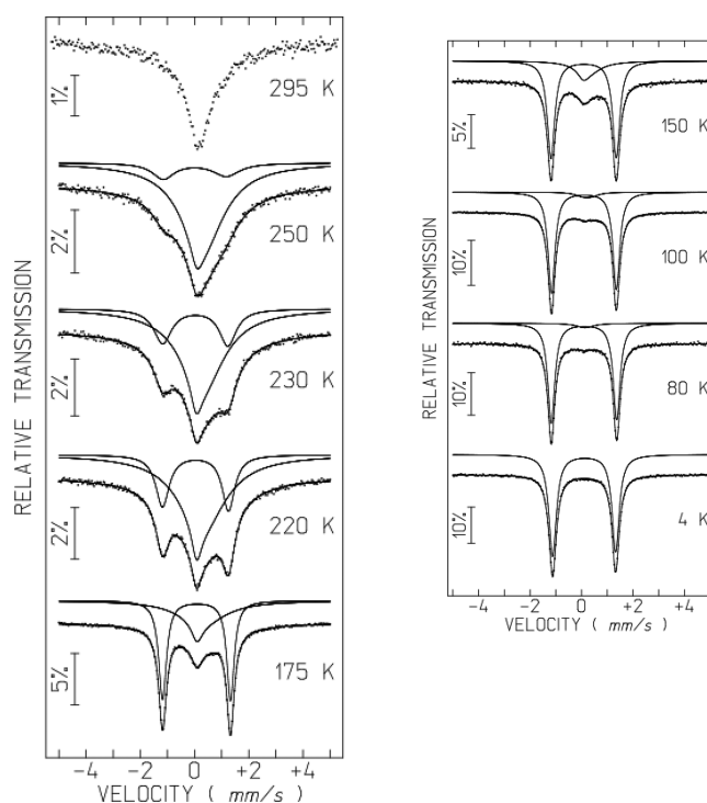
Figure 6. Mössbauer spectra of 1\cdot\text{CHCl}_3 taken at different temperatures. The lines over the experimental points are the sum of two doublets corresponding to HS and LS \text{Fe}^{\text{III}} . The estimated parameters for these doublets are collected in Table 3.
