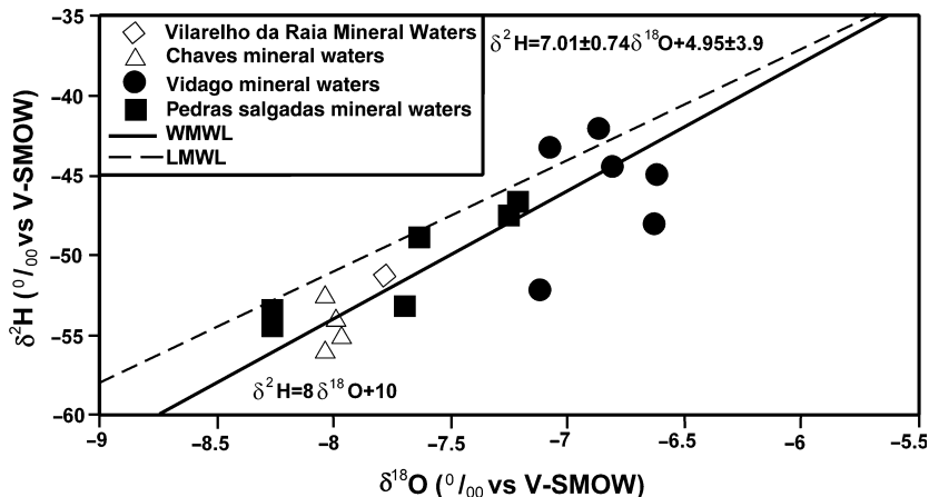
Fig. 3. Plot of \delta^{18}\text{O} versus \delta^2\text{H} (‰ versus V-SMOW) for the hot and cold \text{CO}_2 -rich mineral waters. Modified from Andrade (2003).
