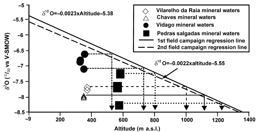
Fig. 6. Determination of recharge elevations of the hot and cold CO 2 -rich mineral waters, from the relationship between \delta^{18}\text{O} of the cold dilute spring and rain waters of the region and elevation. Modified from Andrade (2003).
