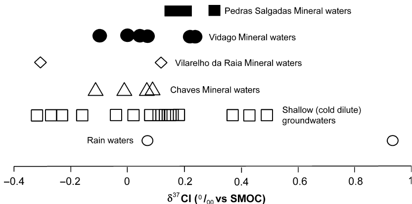
Fig. 10. Range of \delta^{37}\text{Cl} values (‰) versus SMOC) in waters from Vilarinho da Raia–Pedras Salgadas region. Modified from Andrade (2003).
