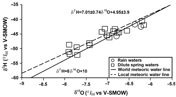
Fig. 4. Plot of \delta^{18}\text{O} versus \delta^2\text{H} (‰ versus V-SMOW) for the cold dilute spring and rain waters of the region. Modified from Andrade (2003).
