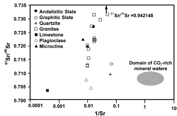
Fig. 9. Plot of 1/Sr versus ^{87}Sr/^{86}Sr for the rocks, minerals and hot and cold CO_2 -rich mineral waters. Sr in mg\ l^{-1} . Modified from Andrade (2003).
