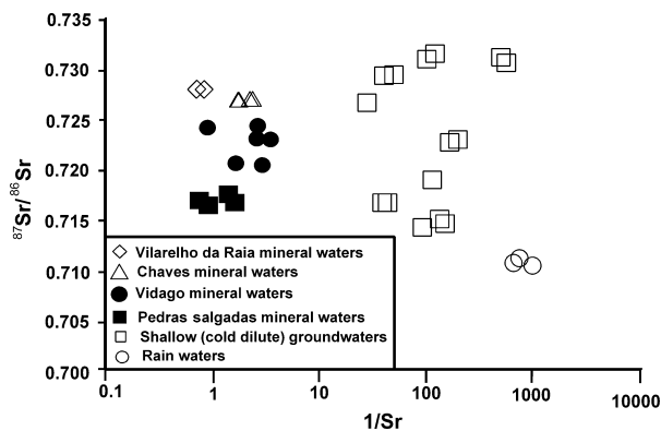
Fig. 8. 1/Sr versus ^{87}Sr/^{86}Sr for the waters from Vilarelho da Raia–Pedras Salgadas region. Sr in mg\ l^{-1} . Modified from Marques et al. (2001a).
