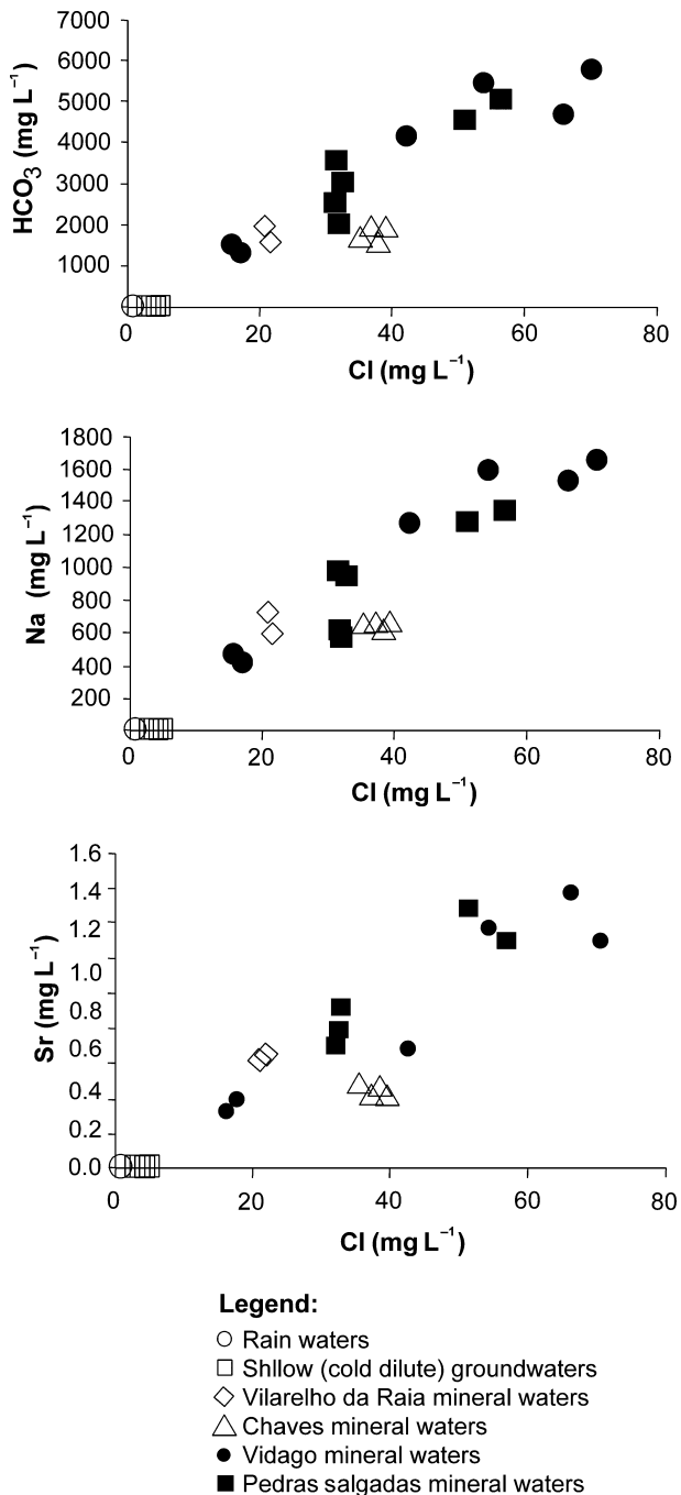
Fig. 2. Cl versus HCO 3 , Cl versus Na and Cl versus Sr (mg l -1 ) for the waters from Vilarelho da Raia–Pedras Salgadas region. (◇) and (△) stands for Type A waters; (●) and (■) stands for Type B waters. Modified from Andrade (2003).
