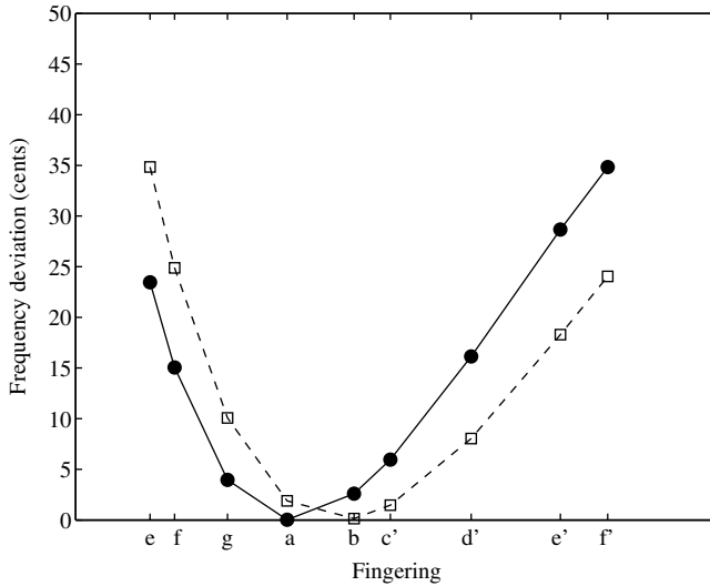
Fig. 20. Frequency deviation associated with the register hole in the case of a real clarinet (i.e. restricting our optimization to fingering from e to f' : above f' , fingerings are modified to ensure the well tuning and the third resonance is used). Optimal positions are \ell_{\star}^{(1)} = 133.7 mm (□) and \ell_{\star}^{(2)} = 145.0 mm (●).
