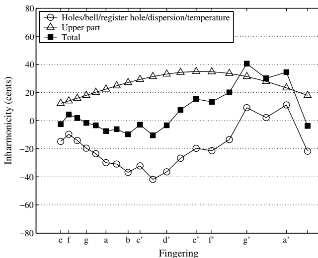
Fig. 16. Inharmonicities due to perturbations found in the upper part (barrel/change in cross-section/upper joint) ( \Delta ), due to hole/bell/register hole/temperature/dispersion ( \circ ), and resulting total inter-register inharmonicity (sum of the two curves) ( \blacksquare ).
