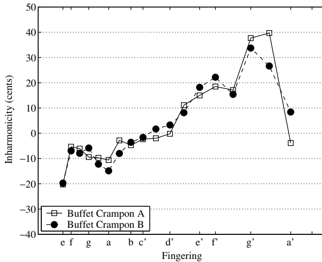
Fig. 15. Measured inter-register inharmonicities obtained from input impedance measurements for two Buffet Crampon clarinet models.
