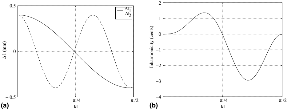
Fig. 6. Length corrections (a) and corresponding inter-resonance inharmonicity (b) for a localized enlargement as a function of k_1 \ell ( \ell' = 10 \text{ mm} , S' = 1.04S ). See Eqs. (31) and (32).
