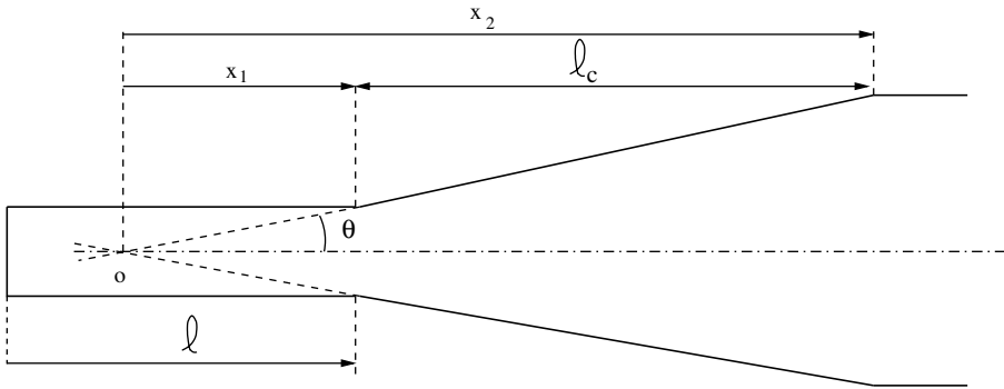
Fig. 8. Geometry and symbols used for the case of a truncated cone.
