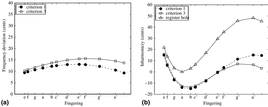
Fig. 23. Frequency deviation for the first register (a) and inter-register inharmonicity (b): localized contraction. Inter-register is improved across the entire register but remains large for the bottom notes.
