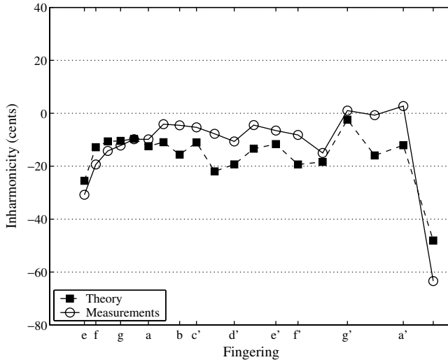
Fig. 13. Inter-resonance inharmonicity. Comparison between input impedance measurements (○) and length correction calculations (■) (uniform temperature).
