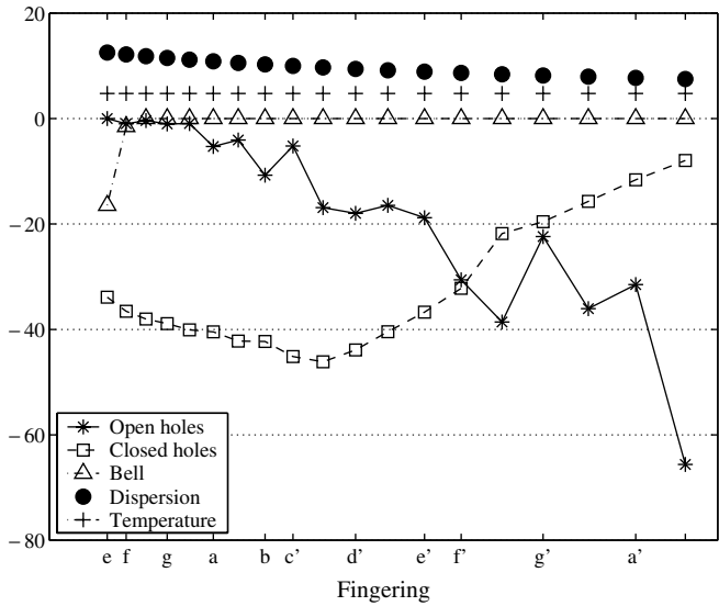
Fig. 11. Inter-resonance inharmonicities due to open holes (*), closed holes (□), dispersion (●), temperature (+) and the flaring bell (△).
