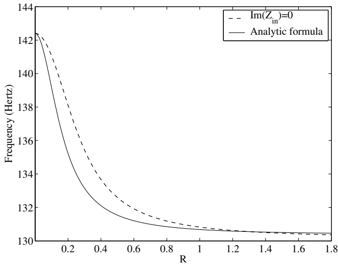
Fig. 25. Playing frequency as a function of the real part of the tone hole impedance ( R = 7.5 mm, r = 4.25 mm, h = 6 mm, \ell_d = 80 mm, L = 0.650 m). In the limit that \mathcal{R} \rightarrow 0 , the frequency of the played tone tends to f_0 , the frequency obtained when the hole is open. In the limit that \mathcal{R} \rightarrow \infty , the frequency of the played tone approaches f_c , the frequency when the hole being closed.
