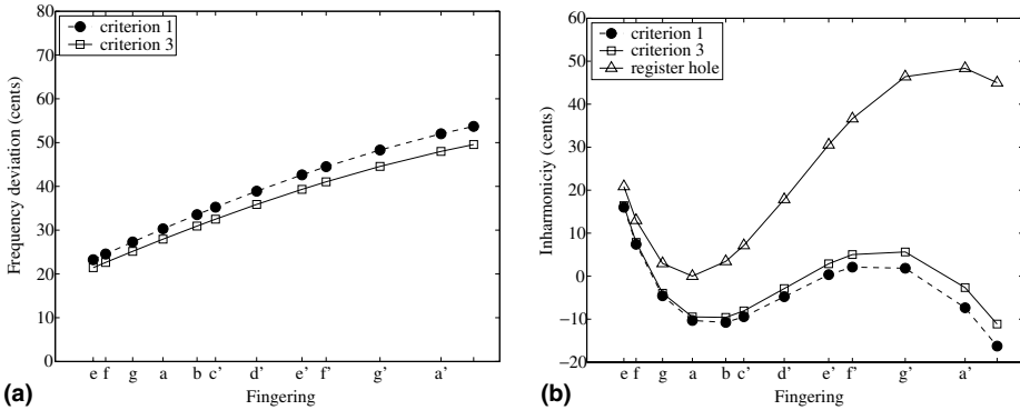
Fig. 21. Frequency deviation for the first register (a) and inter-register inharmonicity (b): abrupt change in cross section area. Minimisations of the two criteria give the same result: the f_2/f_1 -frequency ratio is improved for the highest notes but is still large for the lowest notes.
