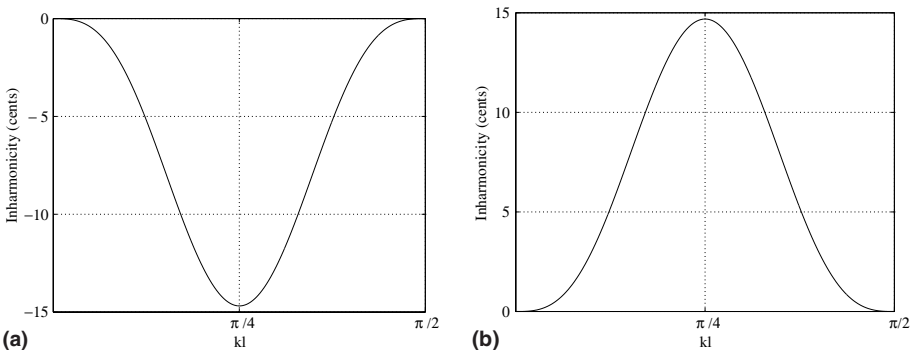
Fig. 7. Inter-resonance inharmonicity due to an abrupt change in cross section area as a function of k_1\ell : contraction S' = 0.98S (a) and enlargement S' = 1.02 (b). See Eqs. (34).
