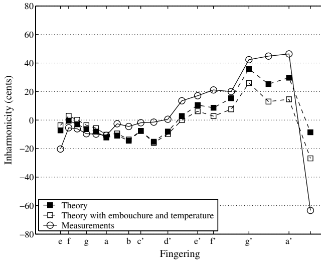
Fig. 14. Inter-register inharmonicity. Comparison between input impedance measurements (○) and length correction calculations (■). Adding the effects of the thermal gradient and the conicity of the embouchure to (■) gives (□).
