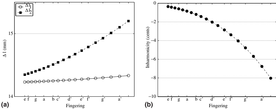
Fig. 4. Length corrections (a) and corresponding inter-resonance inharmonicity (b) for a tone hole of radius r = 4.5 mm, height h = 4 mm, located at a distance \ell_d = 30 mm from the open end for each tube length. See Eqs. (23) and (24).
