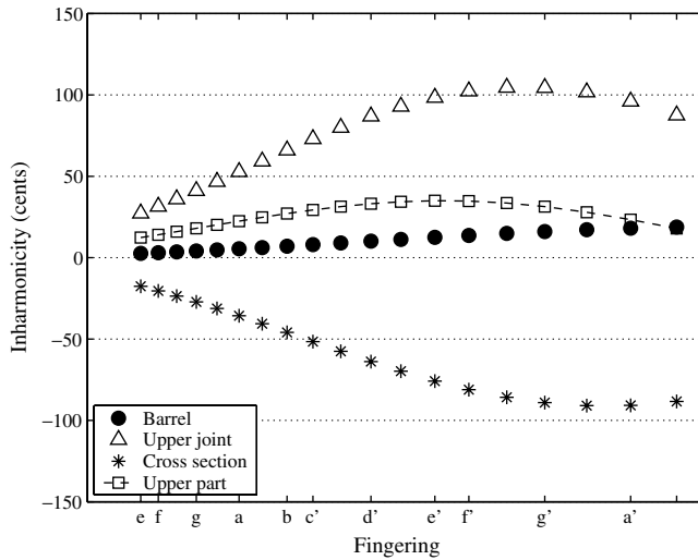
Fig. 12. Inter-resonance inharmonicities due to bore perturbations of the upper part: barrel (●), change in cross sections (*), upper joint (△) and upper part (sum of the three curves) (□).
