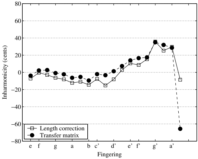
Fig. 10. Total inter-register inharmonicity for a Buffet Crampon clarinet. Length correction calculations (□) and transfer matrix calculations (●) (the temperature gradient has been ignored).
