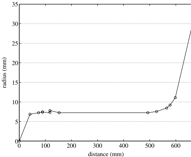
Fig. 2. Radius of a clarinet as a function of the distance from the reed tip (see Table 1).
