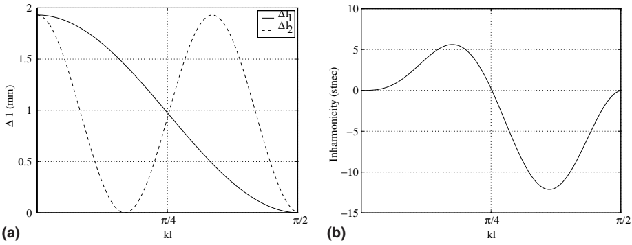
Fig. 5. Length corrections (a) and corresponding inter-resonance inharmonicity (b) for a closed hole whose volume v = 0.3 \text{ cm}^3 as a function of k_1 \ell . See Eqs. (29) and (30).
