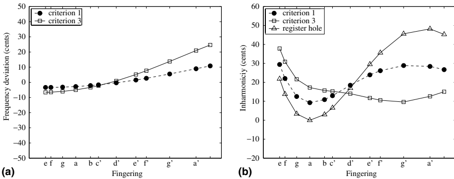
Fig. 22. Frequency deviation for the first register (a) and inter-register inharmonicity (b): localized enlargement. Inter-register inharmonicity gets worse for the lowest notes which is musically unacceptable.
