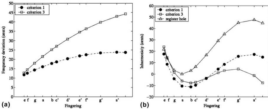
Fig. 24. Frequency deviation for the first register (a) and inter-register inharmonicity (b): positive truncated cone. The f_2/f_1 -frequency ratio is improved globally across the entire scale but it is still 20-cent large for the lowest notes.
