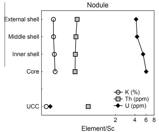
Fig. 9. Distribution of K, Th and U across the aplite nodule.
