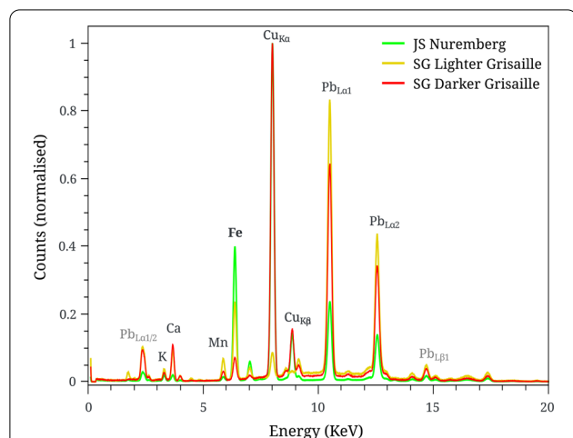
Fig. 7 EDXRF spectra of the two types of grisailles (representative spectra were chosen from Saint Gregory—SG—panel) compared with the spectrum of a Nuremberg Schwarzlot painting on hollow glass signed with the monogram of Johann Schapper, also in Ferdinand II's collection. Values normalised between lighter and darker grisaille by the Ca peak, whilst the whole spectra is normalised to the maximum peak, in the present case being the Cu peak
